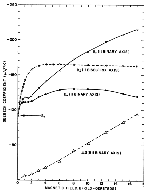
FIG. 1. Seebeck coefficient of bismuth parallel to the threefold axis in a transverse magnetic field at 78°K.
